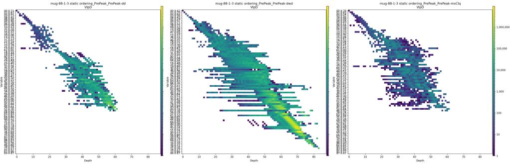
Figure 5: VIPD of forced static ordering on mug88-1-3 , using PREPEAK + ( POAC ) for lookahead, with dd (left), dwd (middle) and mxC1q (right) in the same logarithmic-color scale.
