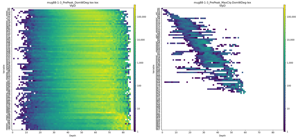
Figure 3: VIPD of search on mug88-1-3, using PREPEAK + (POAC) for lookahead, with dwd (left) and mxClq (right). These graphs use the same logarithmic color scale as Figure 1.
