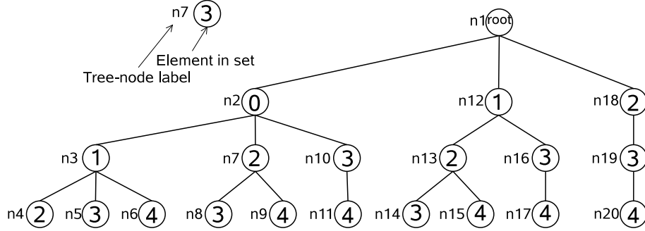
Figure 1: Tree generated by Algorithms 1 and 2 for COMBINATIONS(3, {a,b,c,d,e}) .
